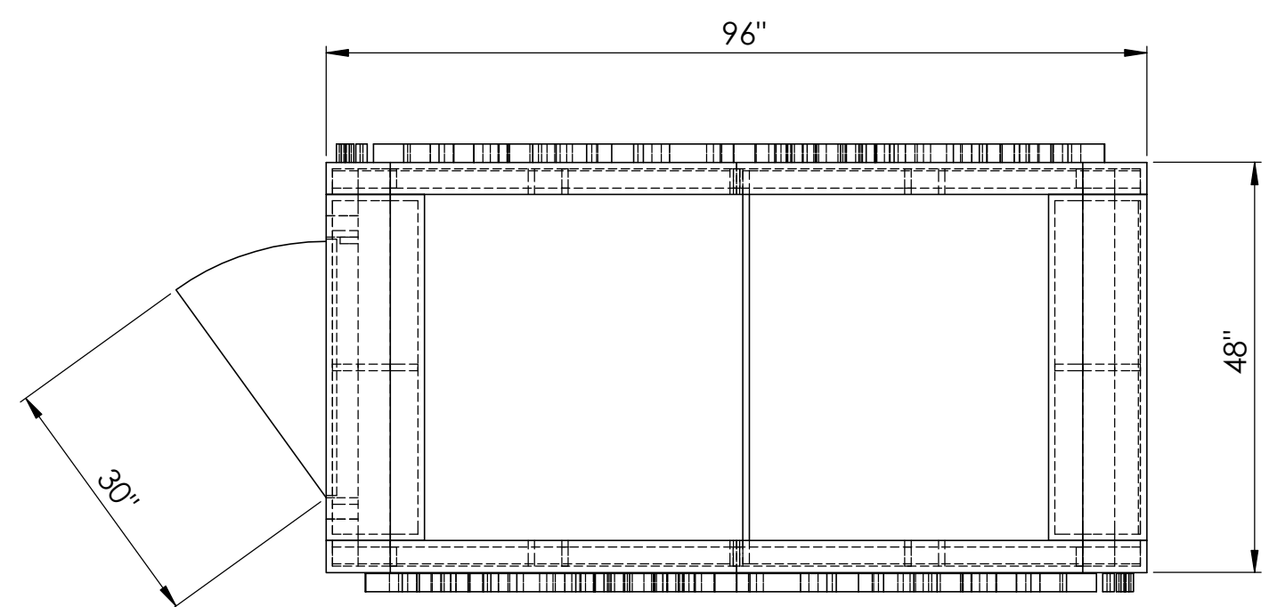
TOP VIEW
