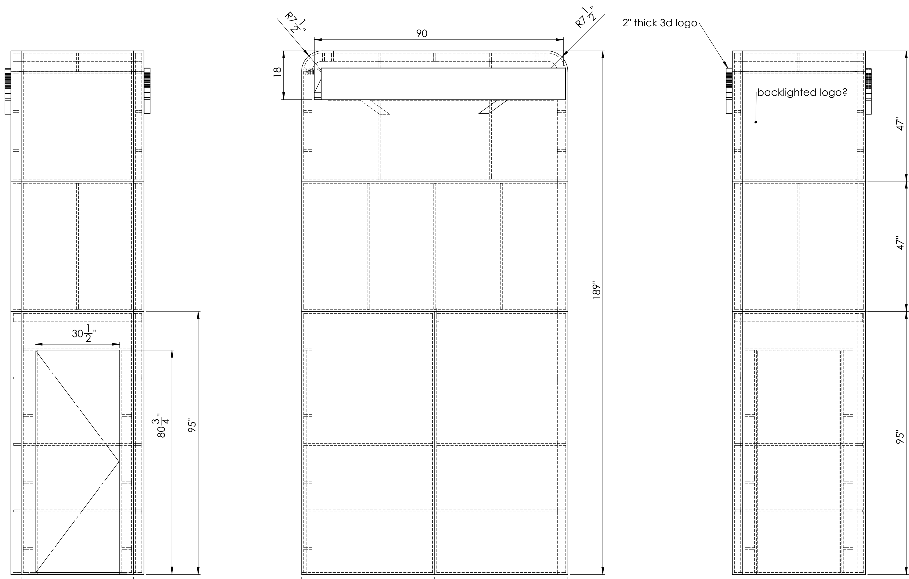
FRONT VIEW TOWER
