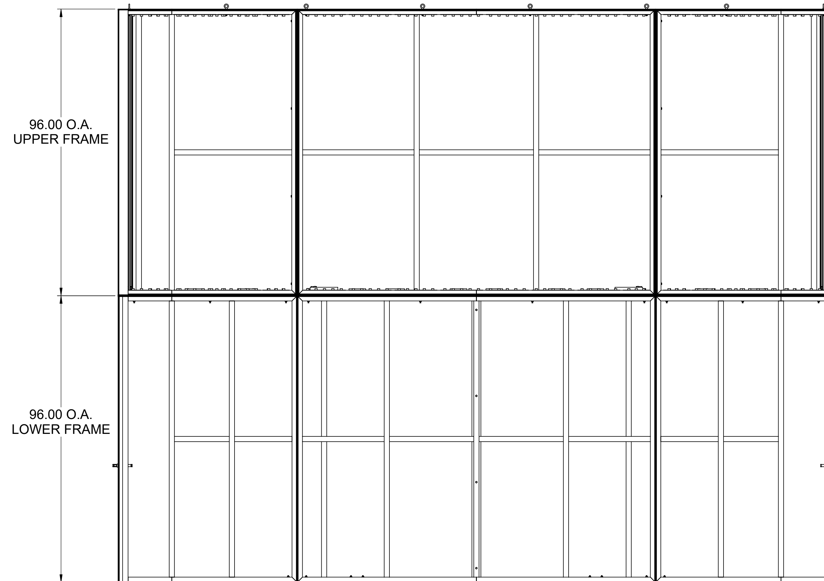
FRONT VIEW
