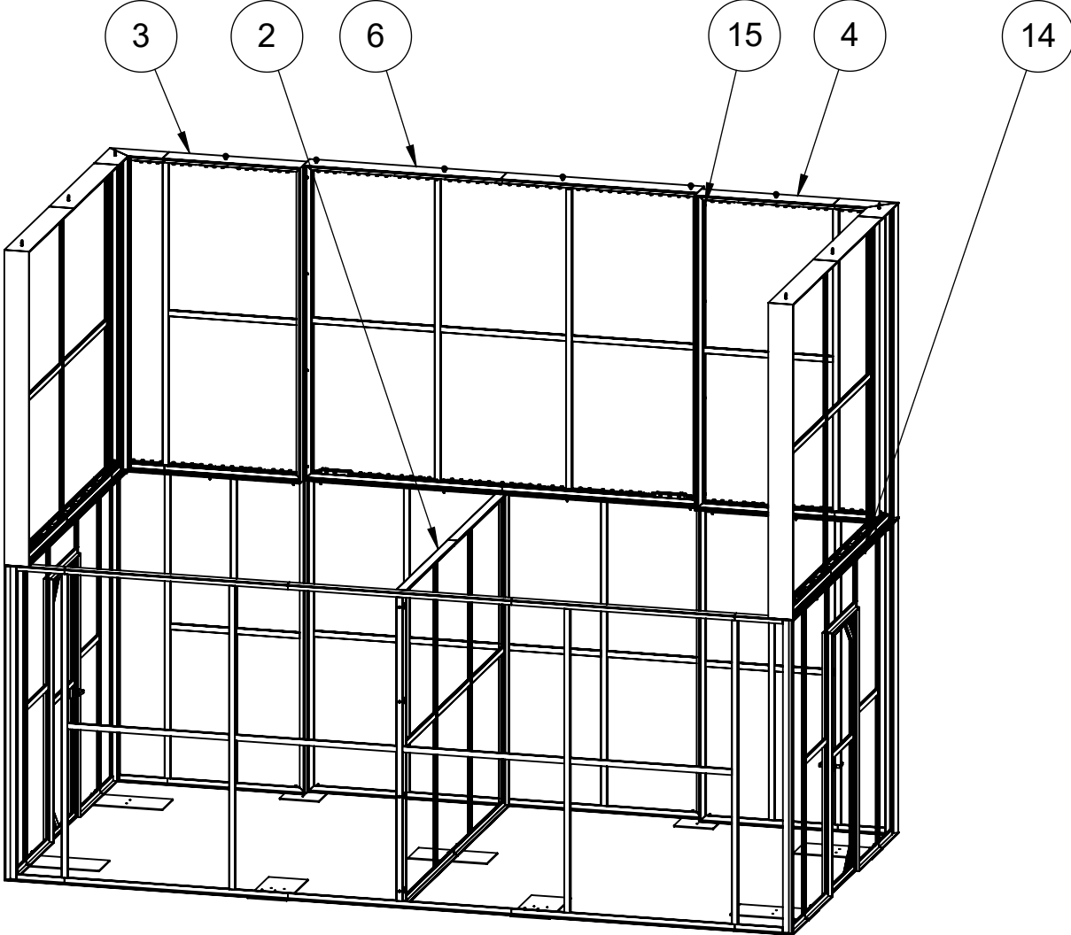
ISOMETRIC VIEW BACK SIDE
