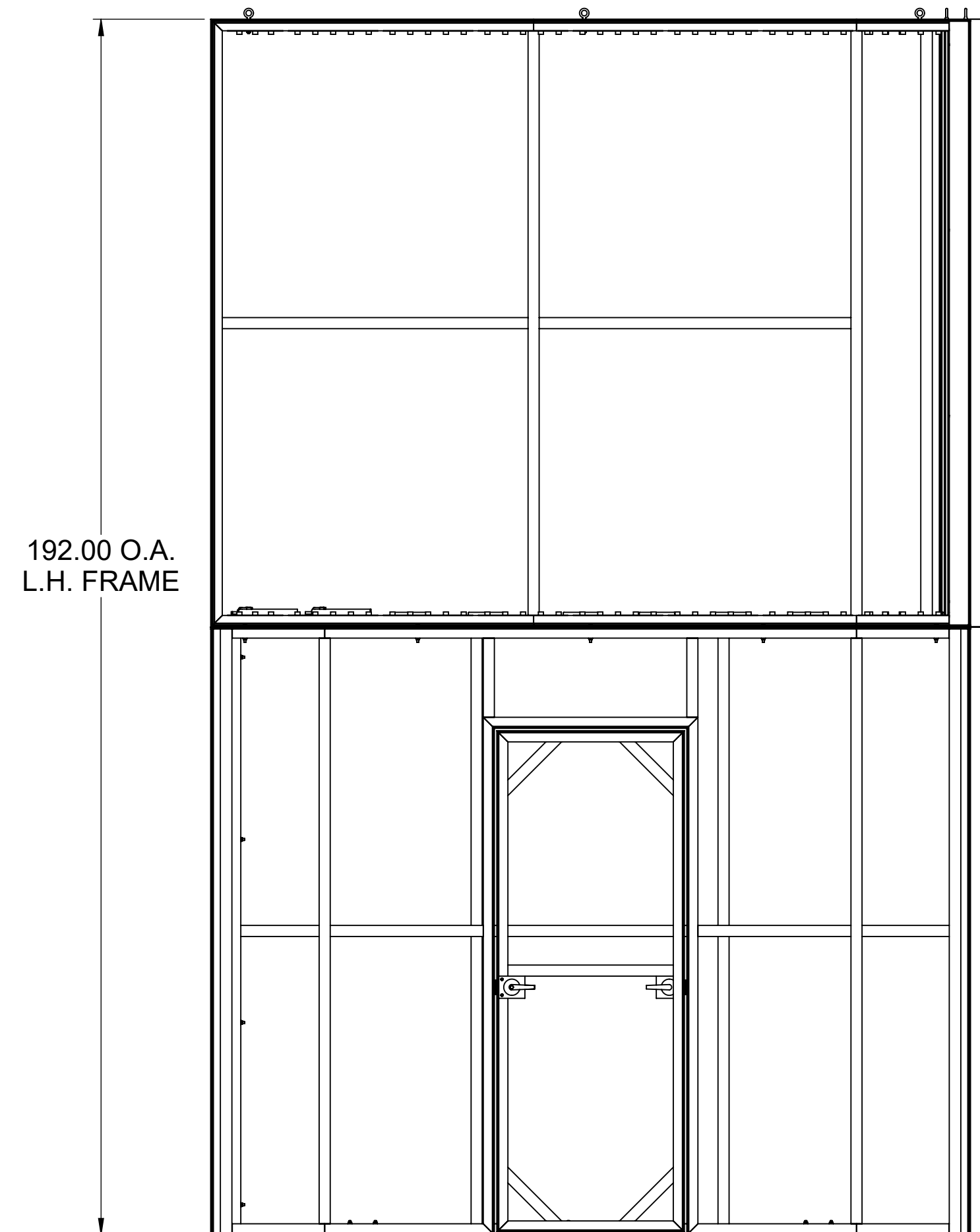
LEFT SIDE VIEW
