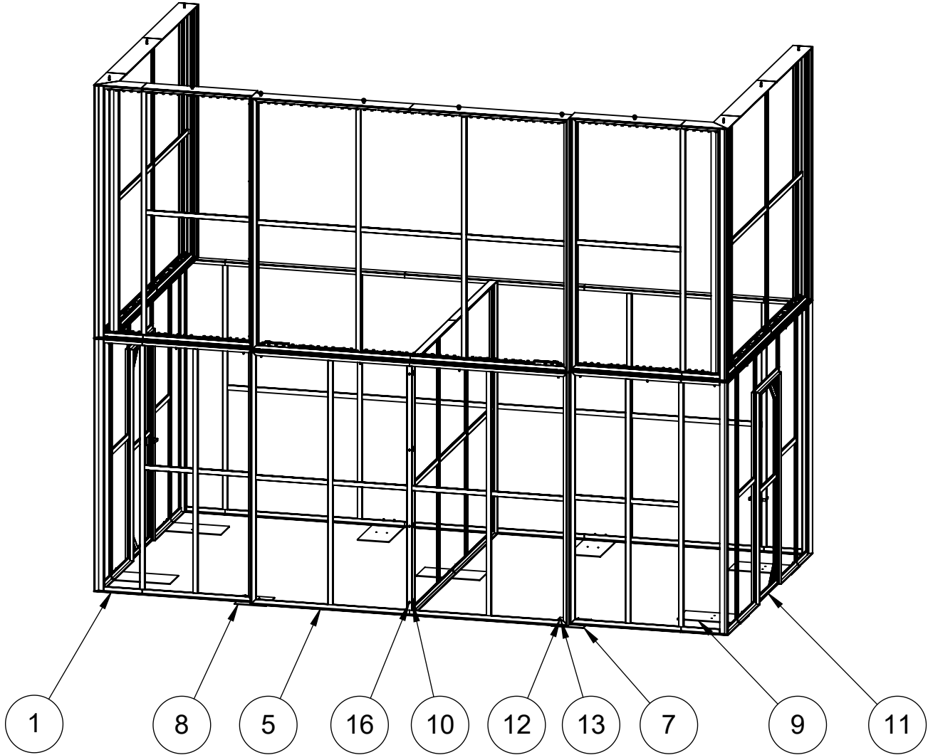
ISOMETRIC VIEW FRONT SIDE
