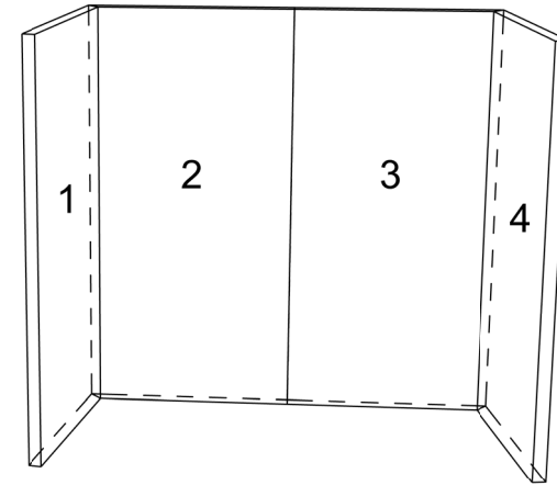
3. ATTACH BACK WALL PANELS TOGETHER
