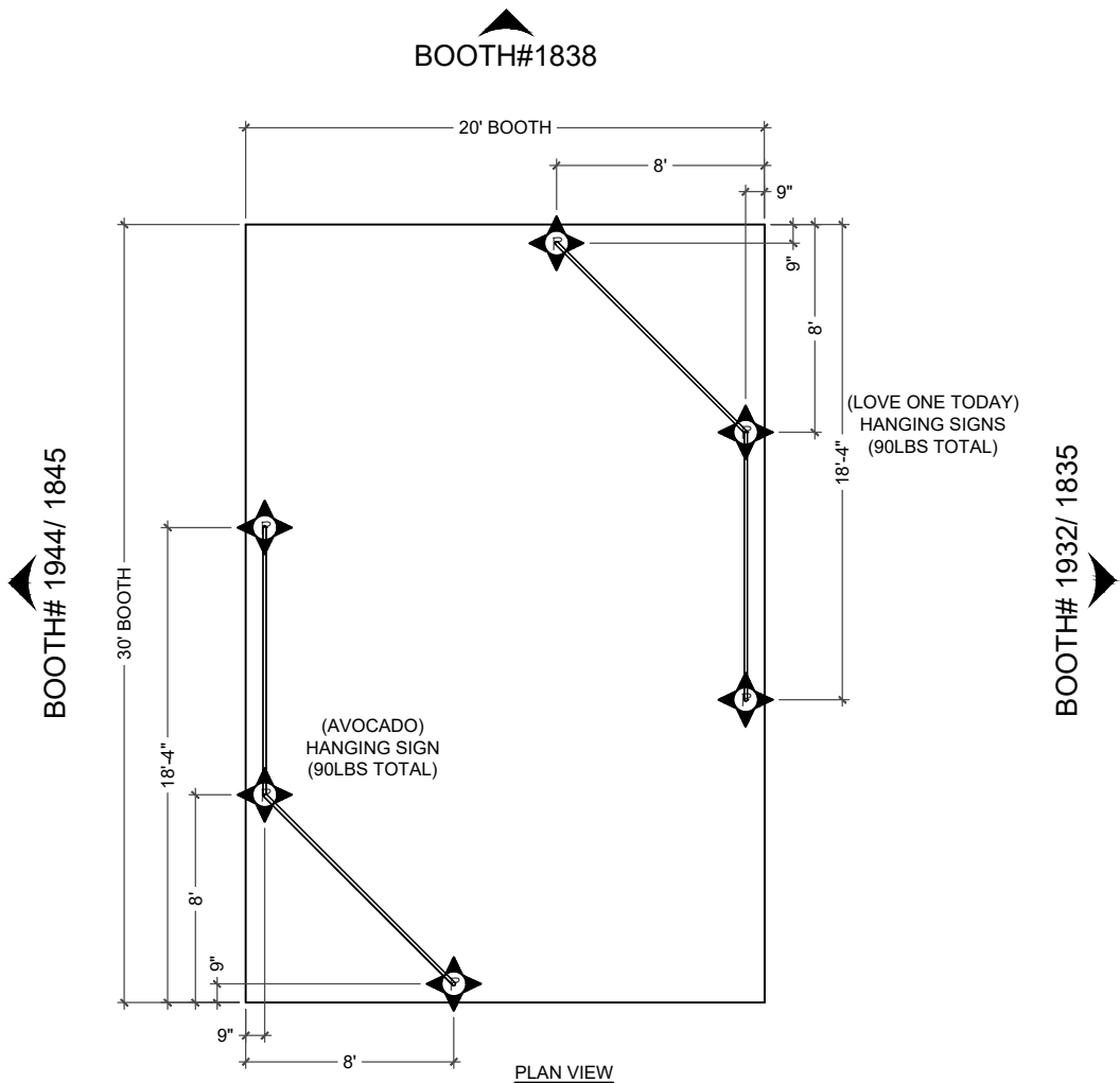
PLAN VIEW
