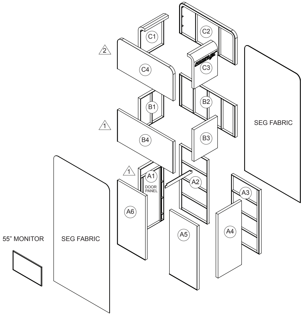
EXPLODED ISOMETRIC: TOWER
