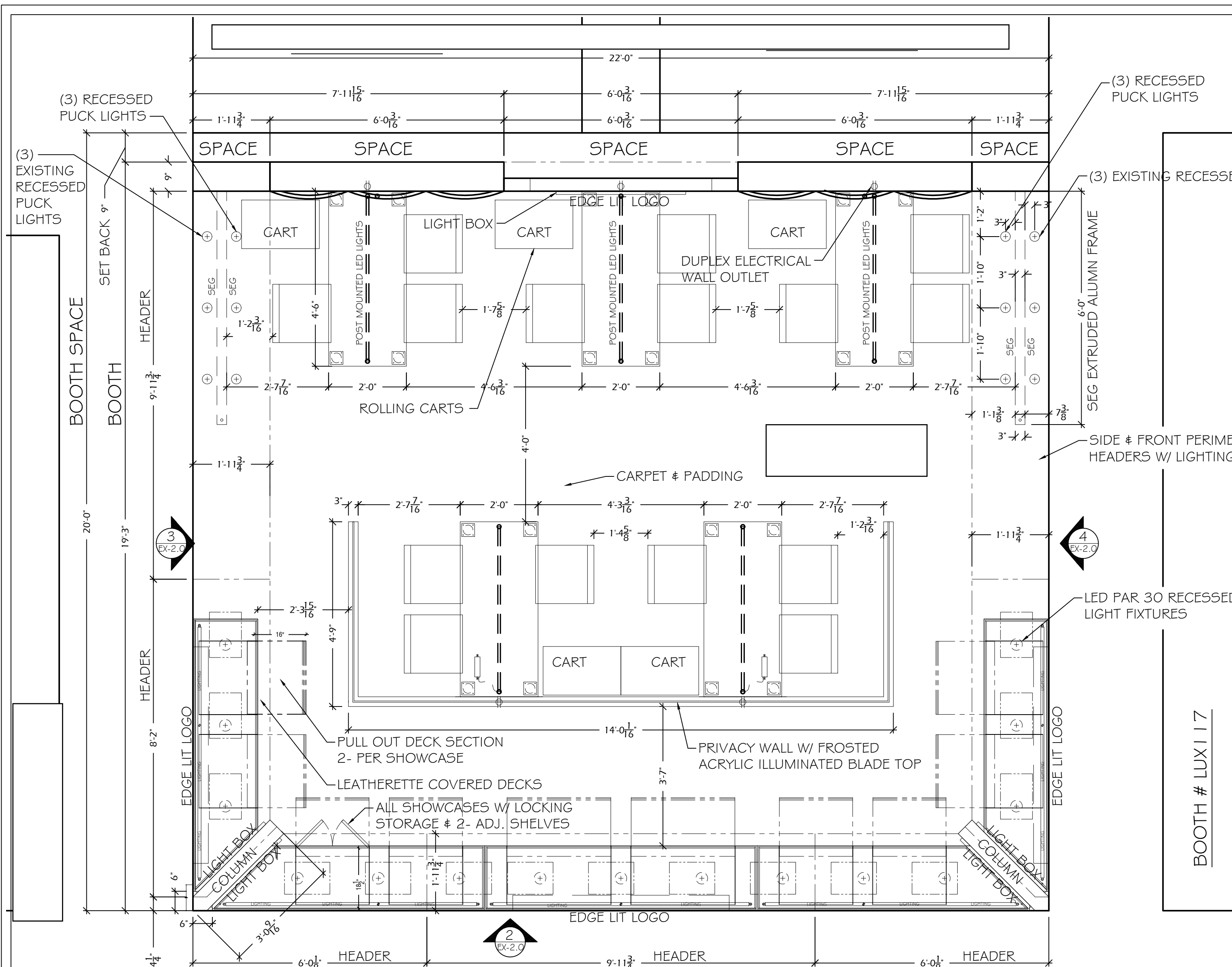
1 FLOOR PLAN SCALE: 1/2"=1'-0"
