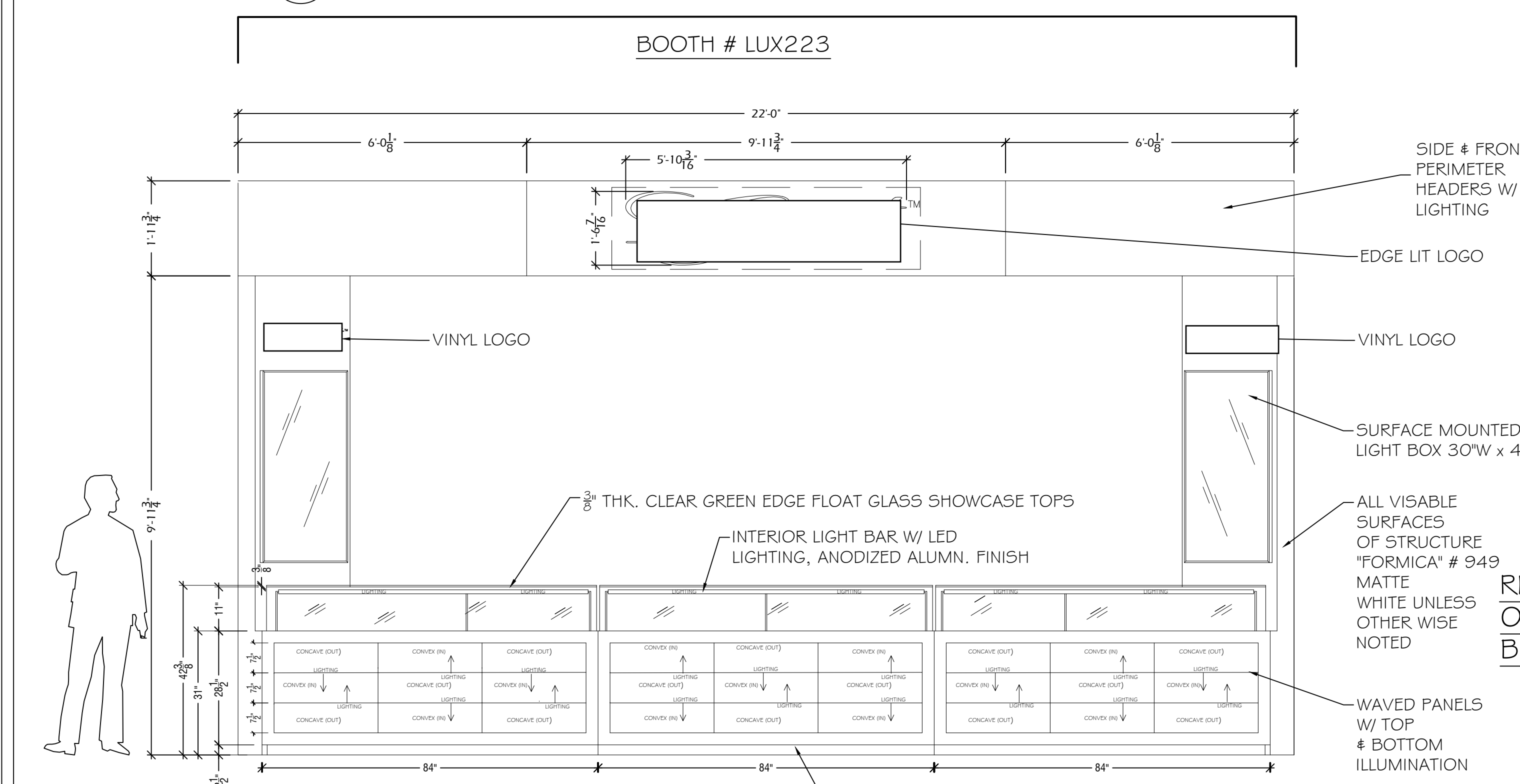
2 FRONT ELEVATION SCALE: 1/2"=1'-0"
