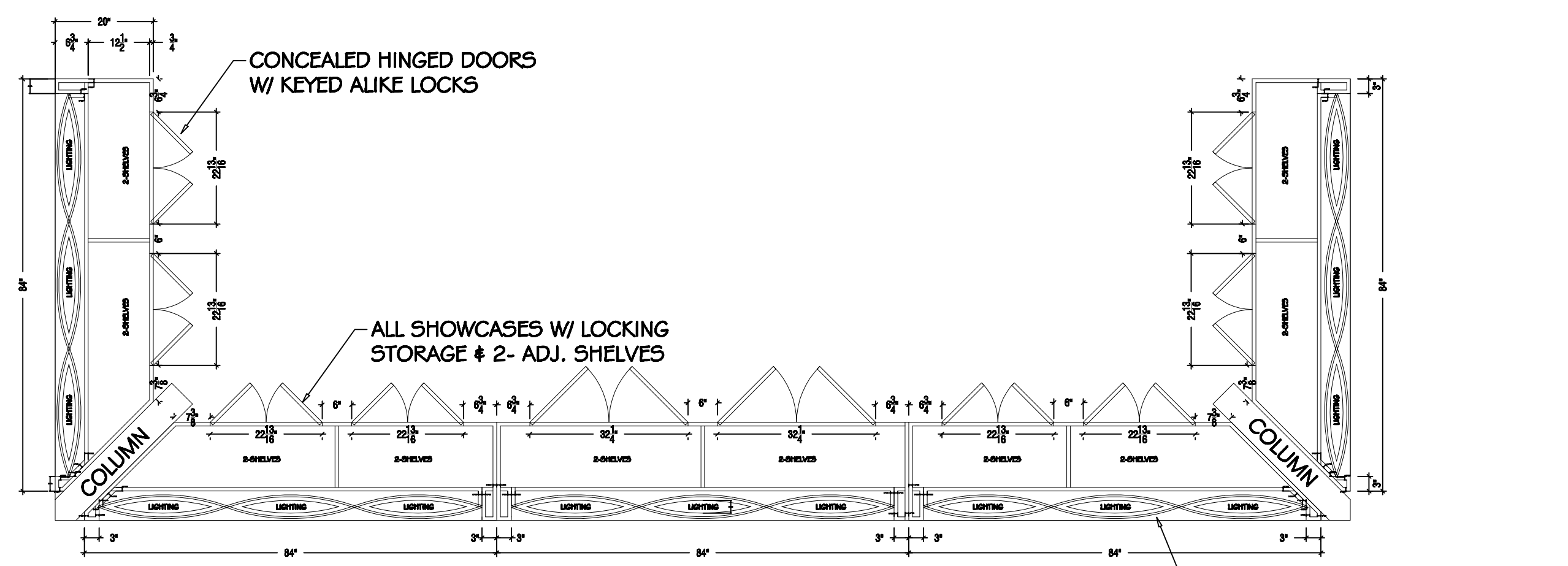
PLAN SECTION: SHOWCASES FRONT OF BOOTH
