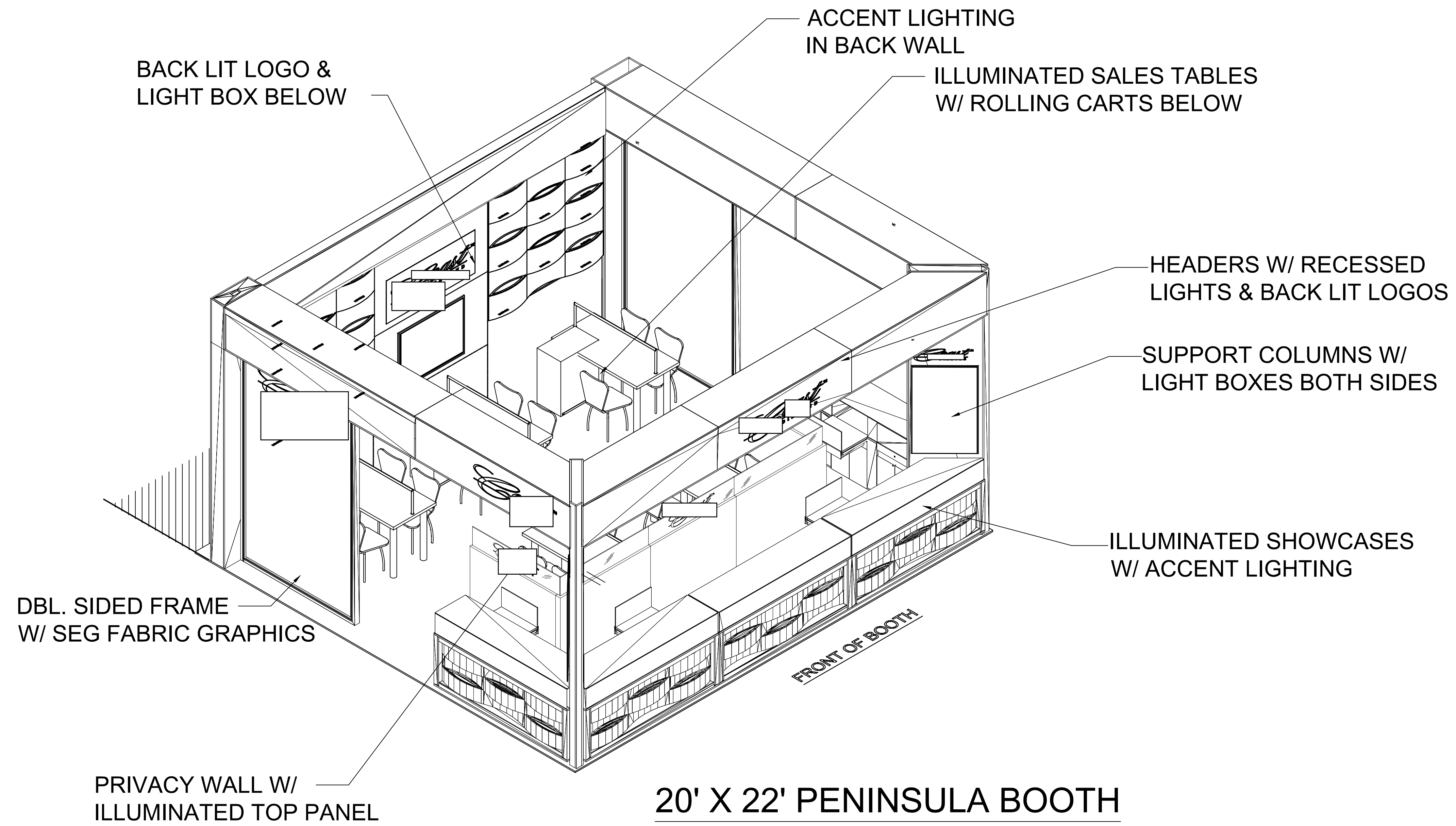
ISOMETRIC VIEW
