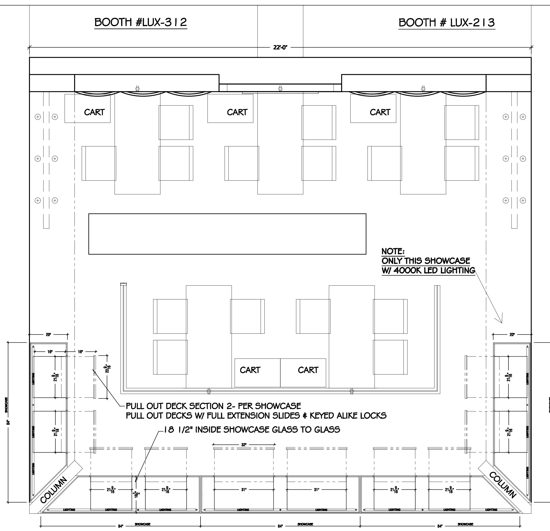
FLOOR PLAN: 22' X 20' PENINSULA BOOTH SPACE FRONT OF BOOTH
