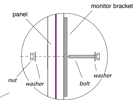
Attach monitor bracket to panel as shown.
