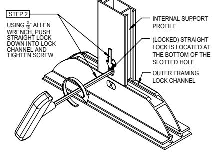
STRAIGHT LOCK CONNECTION SCALE: FULL
