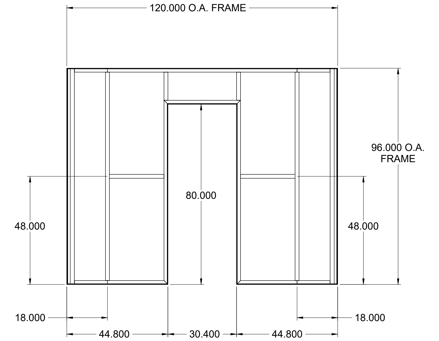
SIDE VIEW
