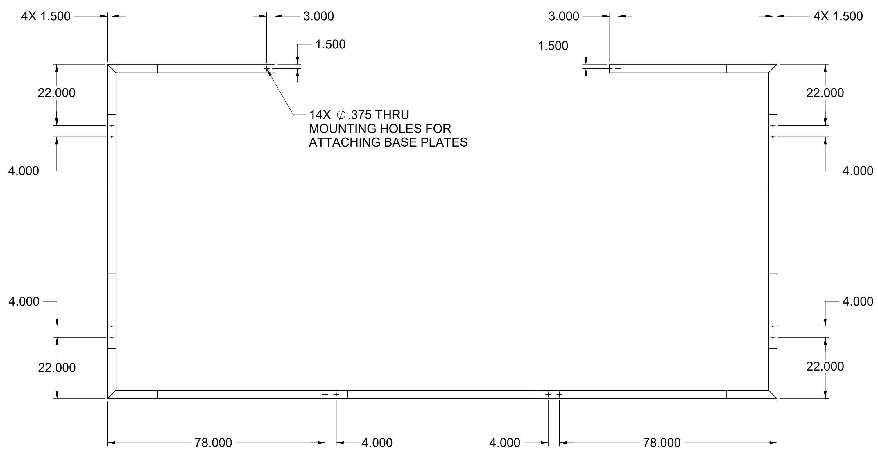
BOTTOM VIEW
