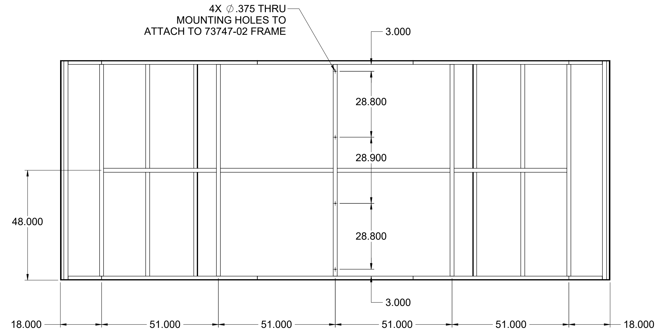
BACK VIEW
