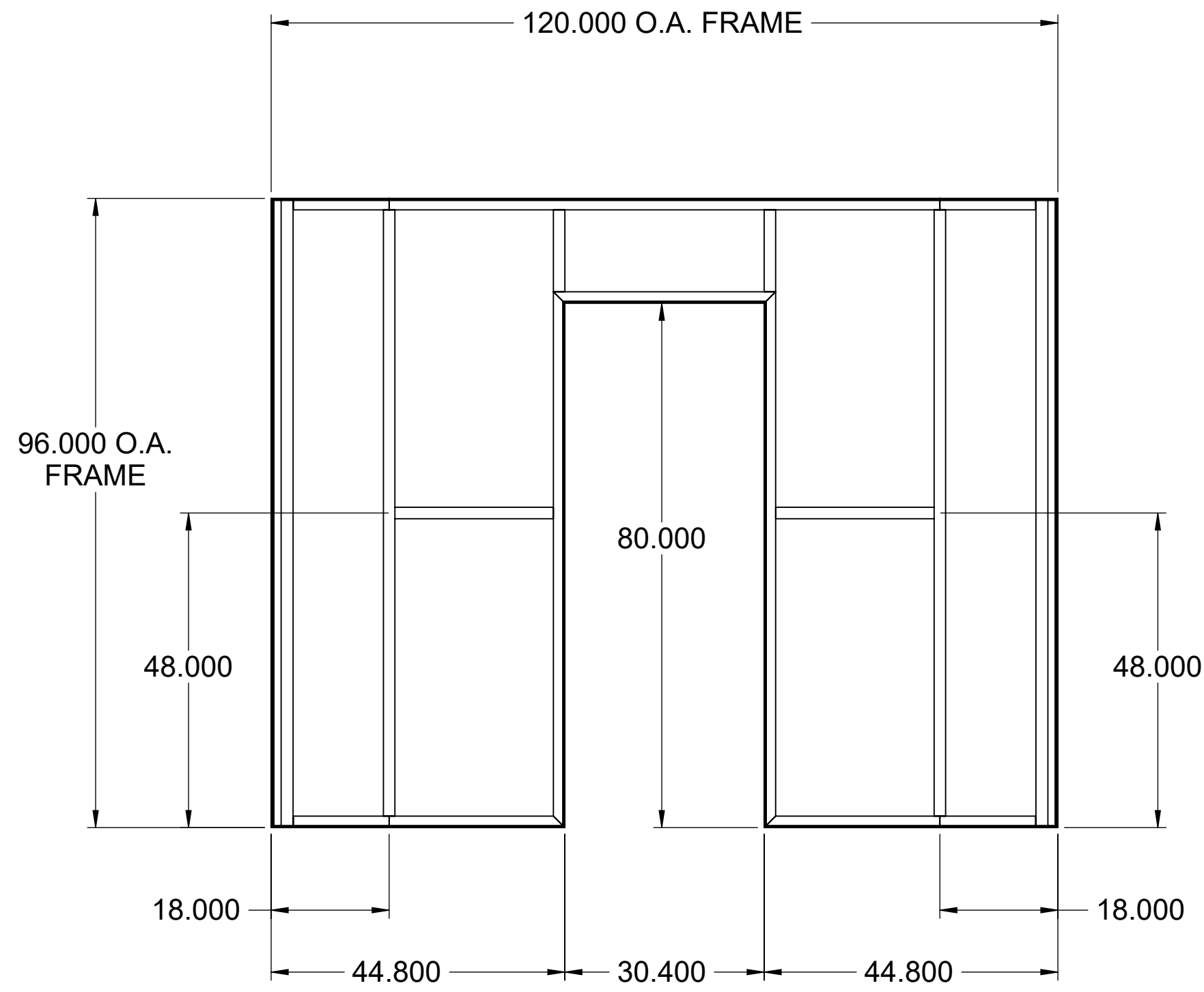
SIDE VIEW
