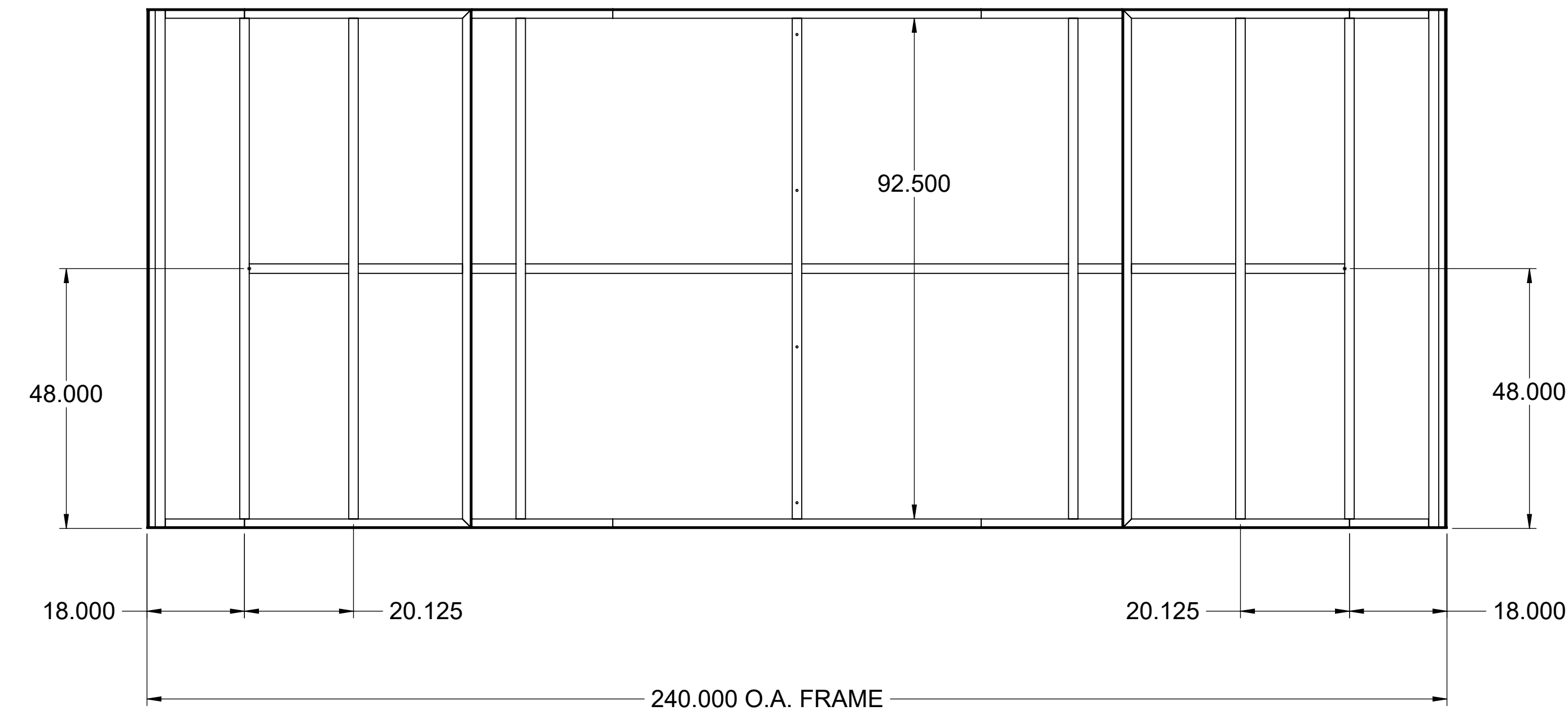
FRONT VIEW
