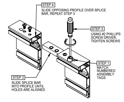
POSITIVE SPLICE LOCK CONNECTION SCALE: FULL
