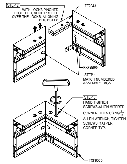
COMPRESSION LOCK CONNECTION SCALE: FULL
