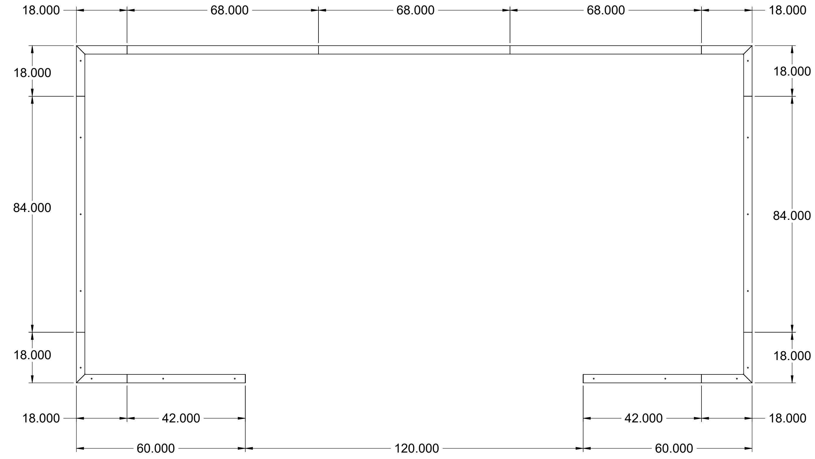
TOP VIEW
