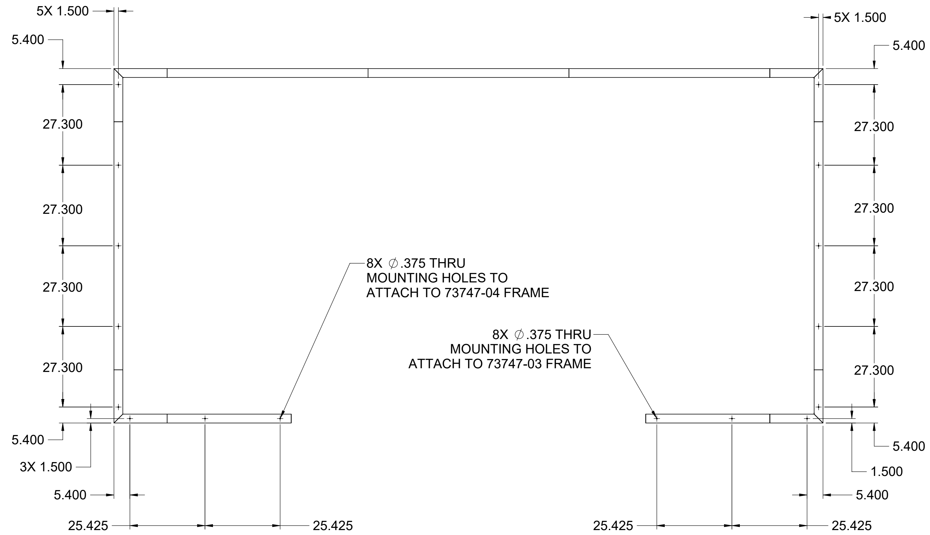
TOP VIEW
